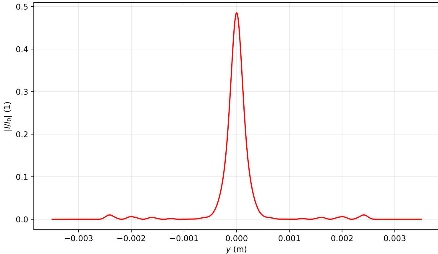
Intensity profile I(x=0, y, z=2.548)/I_0 , \text{Pin}=7.0\text{Pcr} , artificial time
